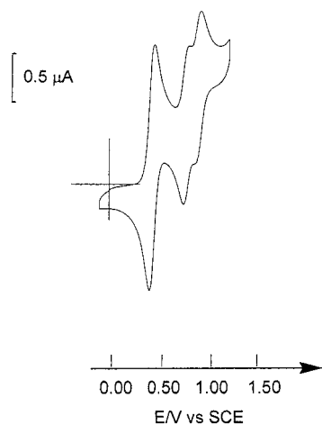
FIGURE 6. CV of 8c in 0.10 M Bu 4 NPF 6 /CH 2 Cl 2 , \nu = 100 \text{ mV s}^{-1} .
