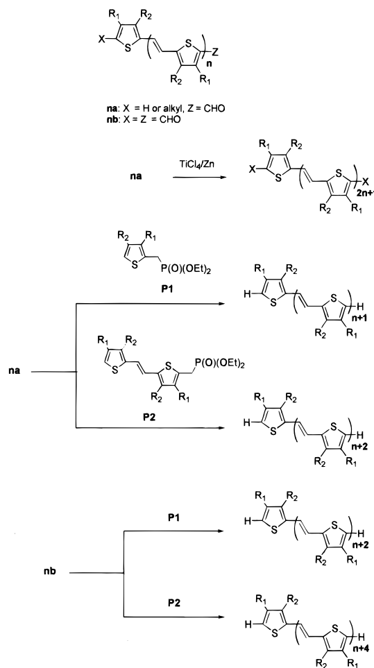
Scheme 1. Synthesis of Soluble n TVs
